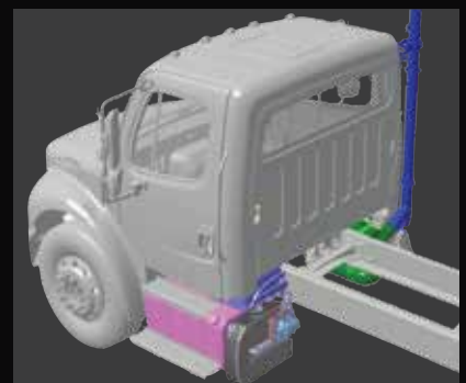
EPA 10 exhaust packaging provides the clear back of cab beverage body builders require, including alternate DEF pump locations.
